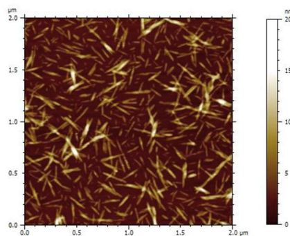
AFM Image (Dispersed in water)
